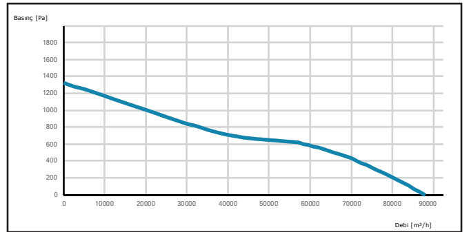
HCTAXI 1120-8-40
